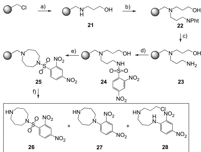
Scheme 5. (a) 3-Aminopropanol, DIEA, 50 °C. (b) N -(3-Bromopropyl)phthalimide, DIEA, 50 °C. (c) N 2 H 4 ·H 2 O, 80 °C. (d) 2,4-Dinitrobenzenesulfonylchloride, 2,6-lutidine, DCM, 23 °C. (e) PPh 3 , DEAD, THF, 23 °C. (f) (i) ACE-Cl, DCE; (ii) MeOH, reflux.
