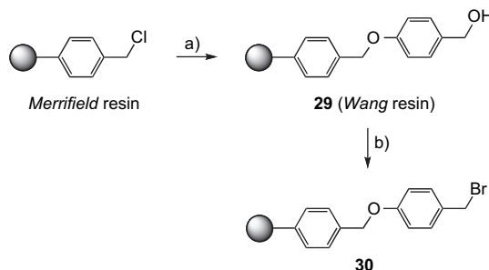
Scheme 6. (a) 4-Hydroxybenzyl alcohol, NaOCH 3 . (b) PPh 3 Br 2 .
