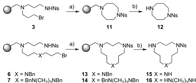
Scheme 2. (a) Cs 2 CO 3 , DMF, 50 °C. (b) (i) ACE-Cl, DIEA, DCE; (ii) MeOH, reflux.
