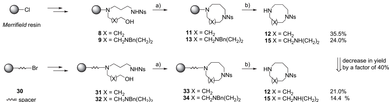
Scheme 7. (a) PPh 3 , DEAD, THF, 23 °C. (b) (i) ACE-Cl, DIEA, DCE; (ii) MeOH, reflux.
