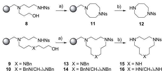
Scheme 3. (a) PPh 3 , DEAD, THF, 23 °C. (b) (i) ACE-Cl, DIEA, DCE; (ii) MeOH, reflux.
