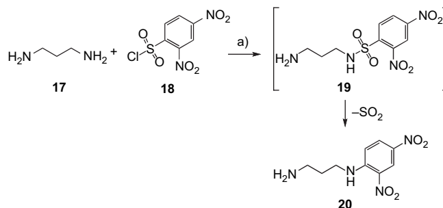
Scheme 4. (a) Et 3 N, CH 2 Cl 2 , 0 °C, evaporation of CH 2 Cl 2 at 23 °C.
